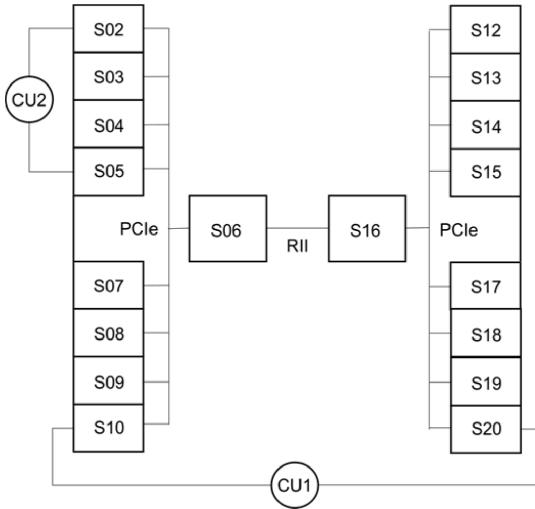
Figure 2. I/O channel path configuration for a representative PCIe I/O drawer in a 8561 and 3907 model
